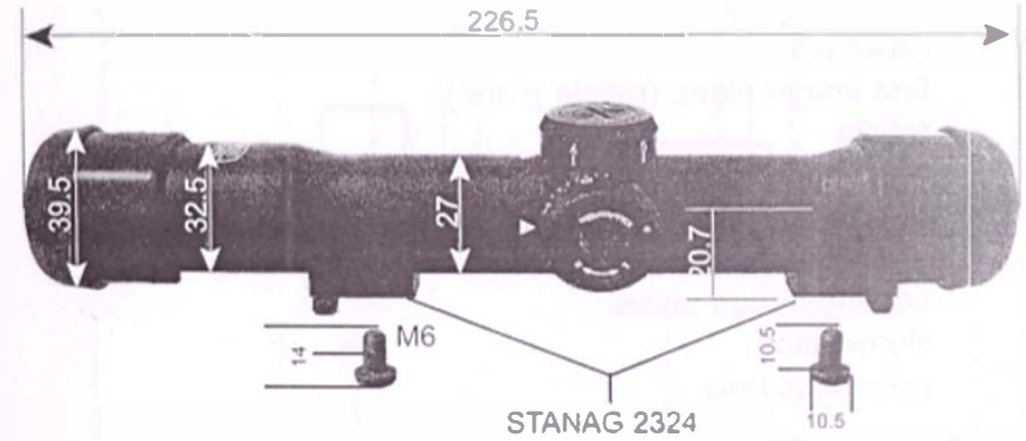
Fig. 1 Main dimensions of the unit
